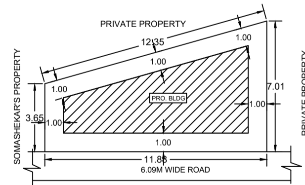
SITE PLAN
